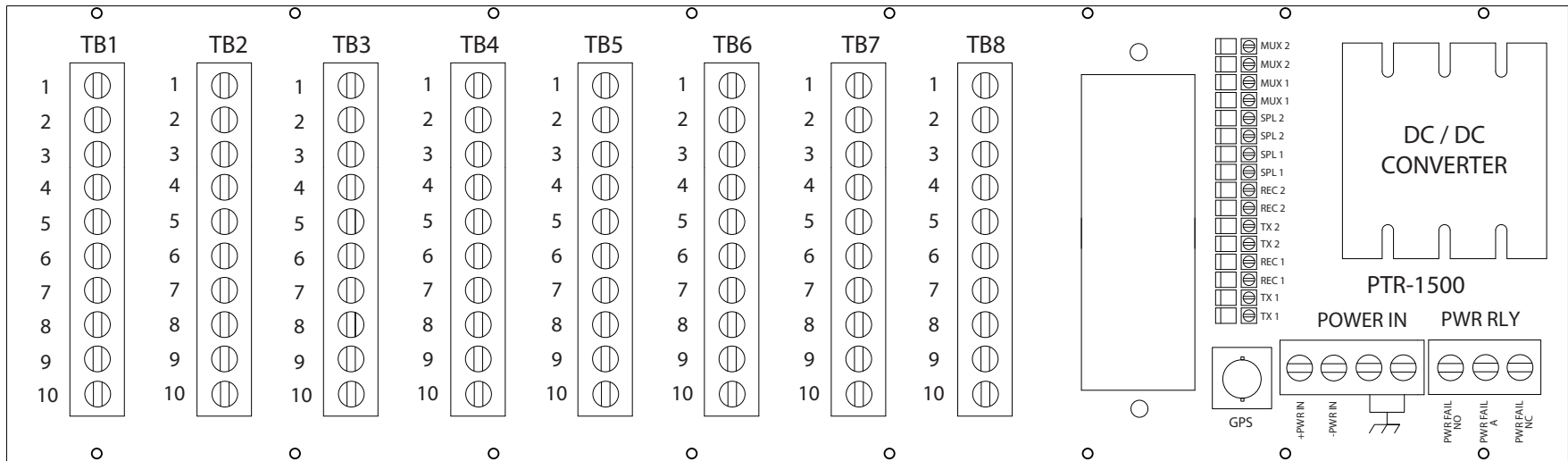
PTR-1500 Standard Configuration Rear View
